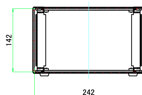
B-B (1:5)
