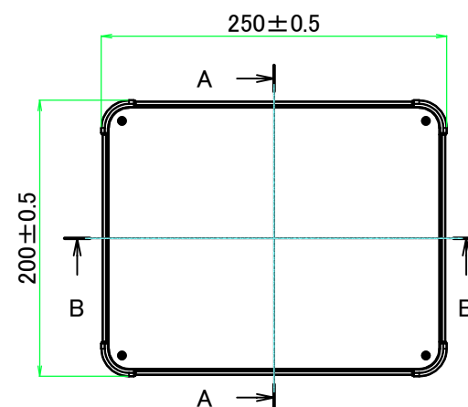
E view
